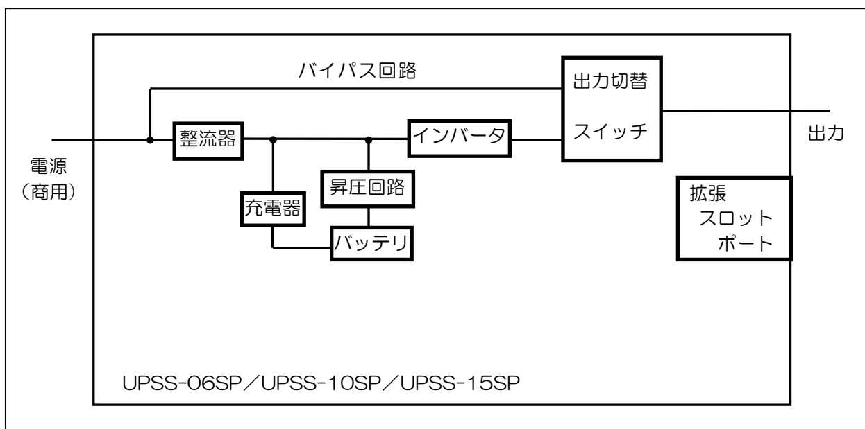
UPSS-06SP/UPSS-10SP/UPSS-15SP 概略構成図
