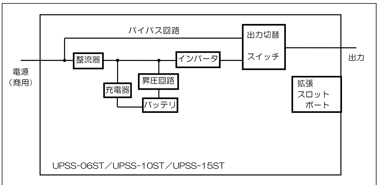
UPSS-06ST/UPSS-10ST/UPSS-15ST 概略構成図
