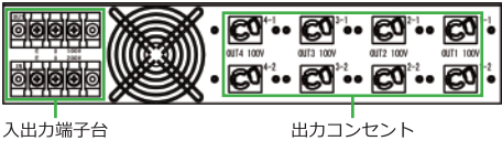
UPSS-ITRD-5K2UIR (5kVA)
